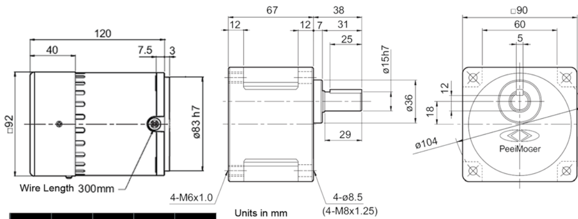
Figure 9: Dimensions for ACP-M-5IK60N-(A)(C)(S)FUV
