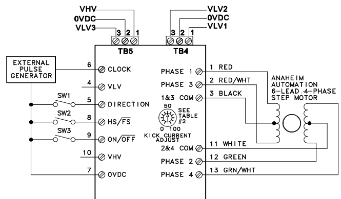
FIGURE 3: HOOKUP DIAGRAM.
