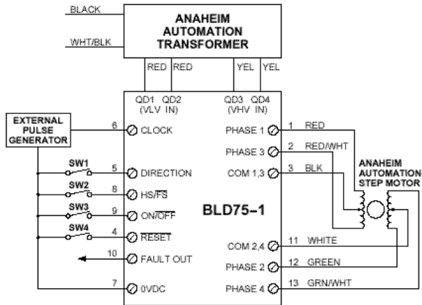
Figure 5: Hook Up Drawing
