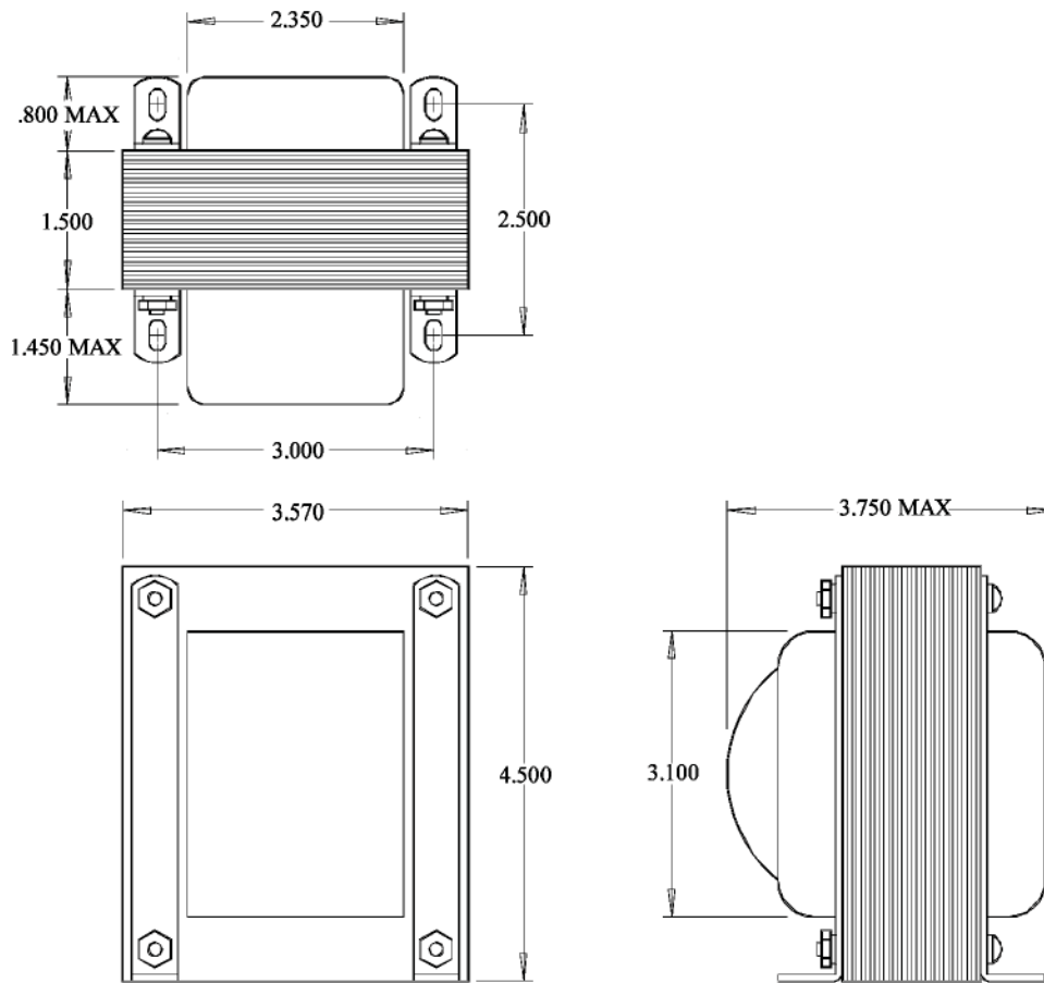
Figure 6: Transformer Dimensions
