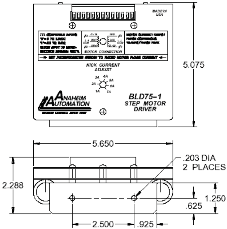
Figure 10: BLD75-1 Dimensions
