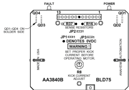
Figure 4: Jumper Location Drawing
