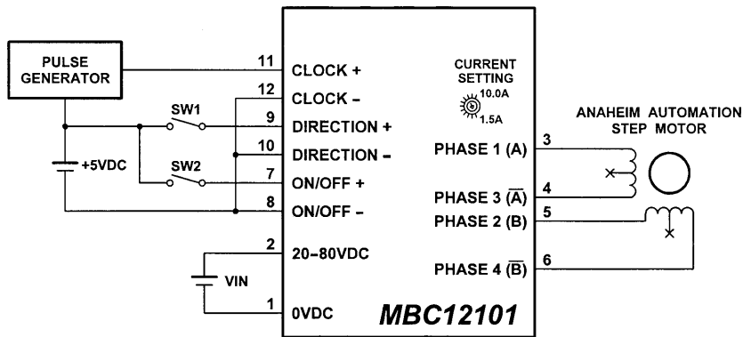
Figure 3: Hook up for current sourcing inputs
