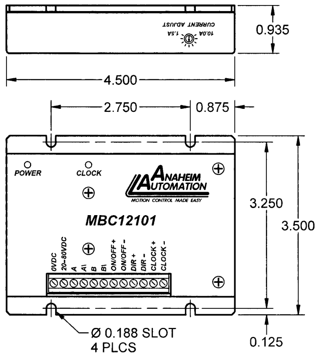
Figure 5: MBC12101 dimensions
