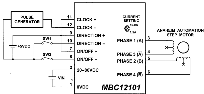
Figure 4: Hook up for current sinking inputs
