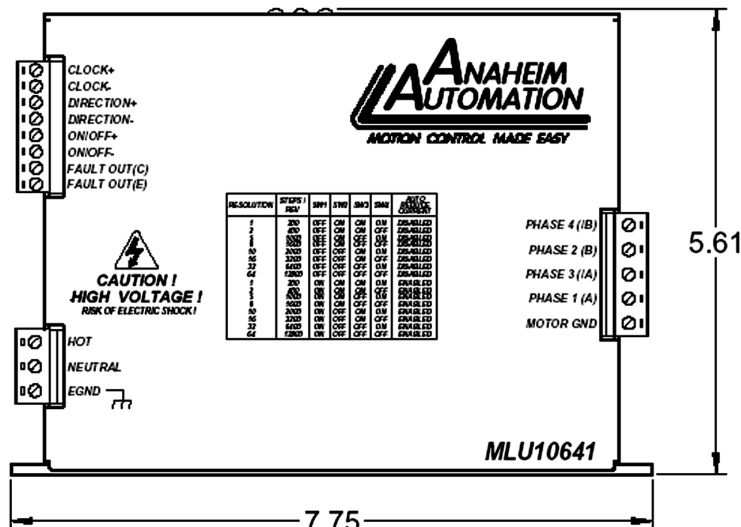
Figure 1: MLU10641 Dimensions
